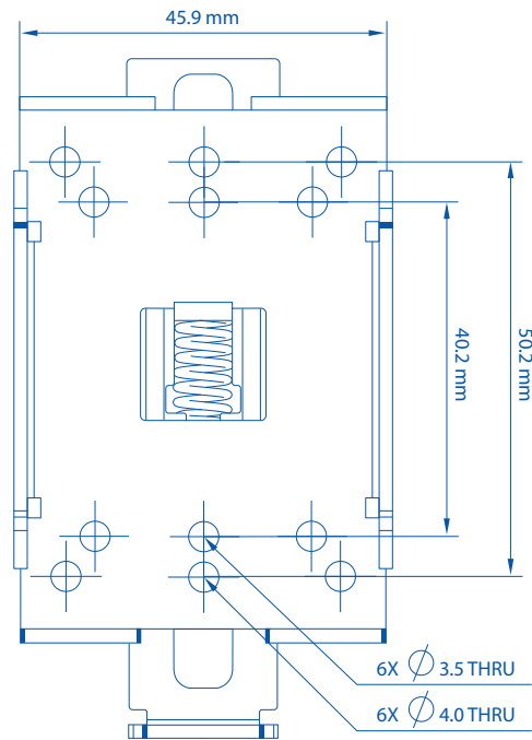
BOTTOM VIEW
