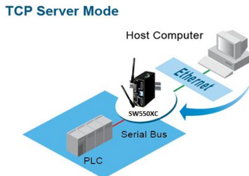
Figure 5.2 An Example of TCP Server Link Mode
