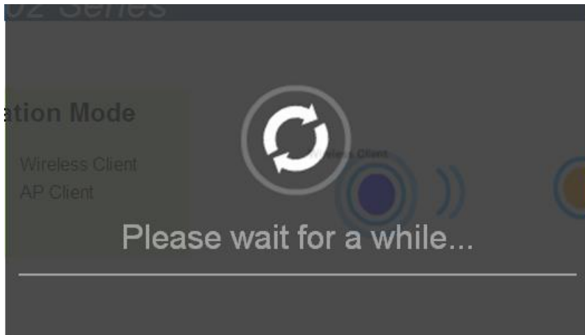
Figure 4.15 Waiting Message
