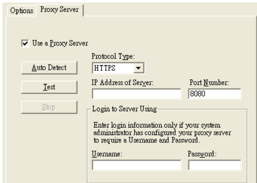
Figure 6.19 Proxy Server Tab under Serial/IP Advanced Settings
